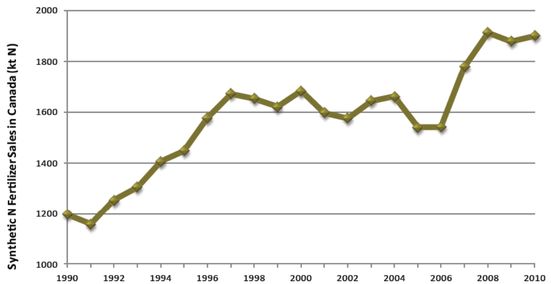
Figure A3-3 Synthetic Nitrogen Fertilizer Sales in Canada from 1990 to 2010
