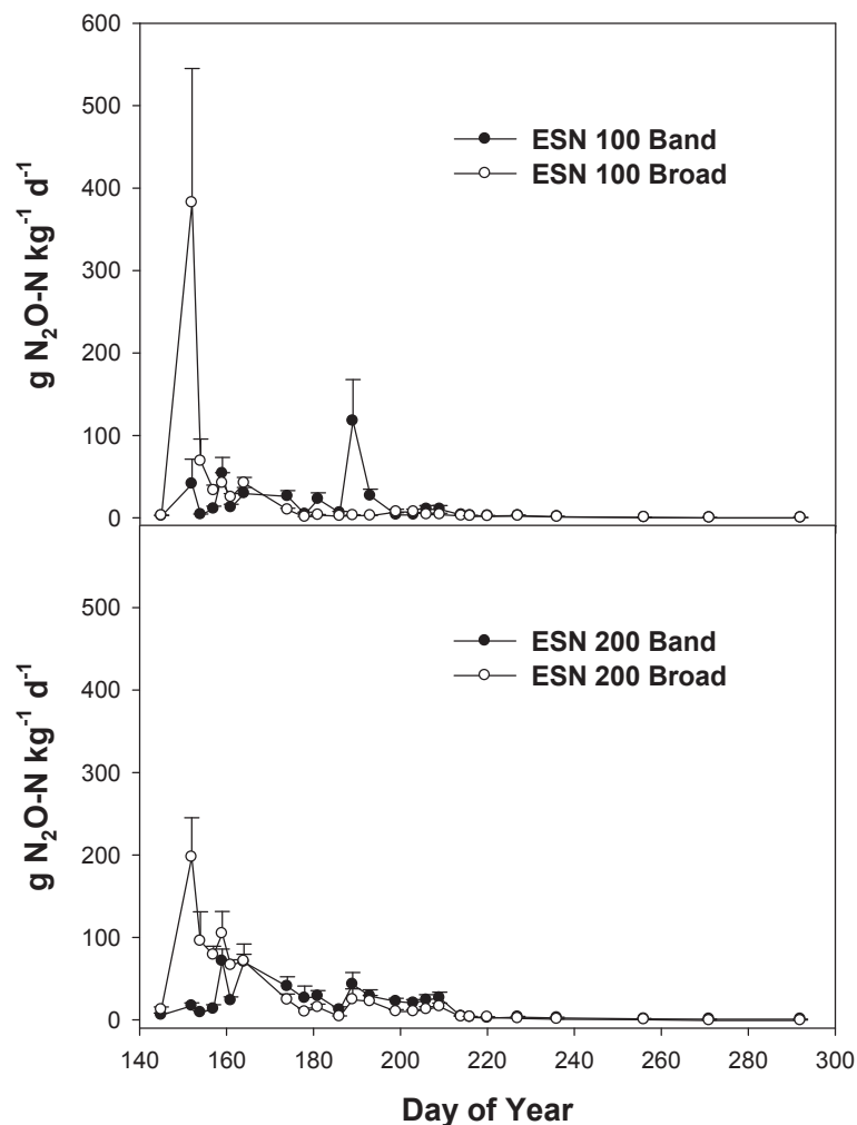
Figure 8. Potato Placement: Emission of nitrous oxide in 2011 from the AESB-Carberry N Placement Study planted to Russet Burbank under irrigation. Treatments shown are, ESN 100 Broad and ESN 100 Band as 100 kg N ha -1 broadcast incorporated following application at hilling and single application banded to the side of seed tubers, respectively, as well as ESN 200 Broad and ESN 200 Band as 200 kg N ha -1 broadcast incorporated following application at hilling and single application banded to the side of seed tubers, respectively. Means are for 16 chamber locations for each treatment \pm 1 standard error of the mean.
