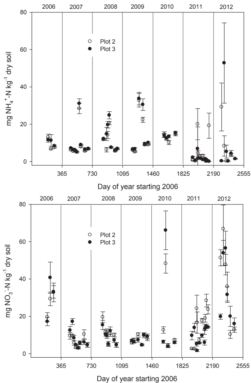
Figure 2. Fall vs. Spring: Extractable \text{NH}_4^+ and \text{NO}_3^- from soil for Plot 2 and 3 at the TGAS-MAN study site.
