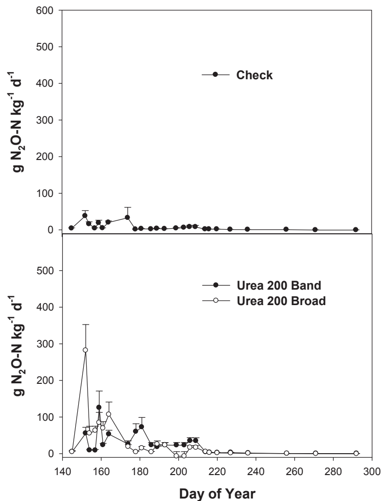
Figure 7. Potato Placement: Emission of nitrous oxide in 2011 from the AESB-Carberry N Placement Study planted to Russet Burbank under irrigation. Treatments shown are, Check (0 kg N ha -1 ), and Urea 200 Broad and Urea 200 Band as 200 kg N ha -1 broadcast incorporated following application at hilling and single application banded to the side of seed tubers, respectively. Means are for 16 chamber locations for each treatment \pm 1 standard error of the mean.
