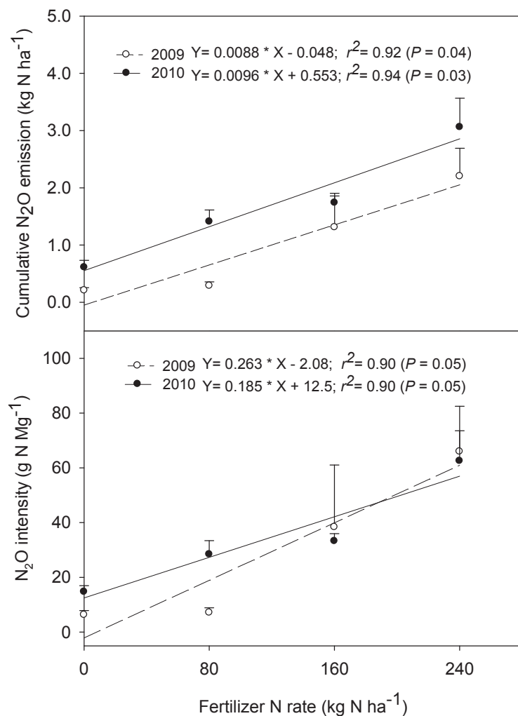
Figure 4. N Rate: Growing season cumulative N 2 O emissions and yield based N 2 O intensity as a function of fertilizer N rate in 2009 and 2010. Bars indicate +1 standard error (n = 8 for cumulative N 2 O emission and n = 4 for N 2 O intensity) of the mean.
