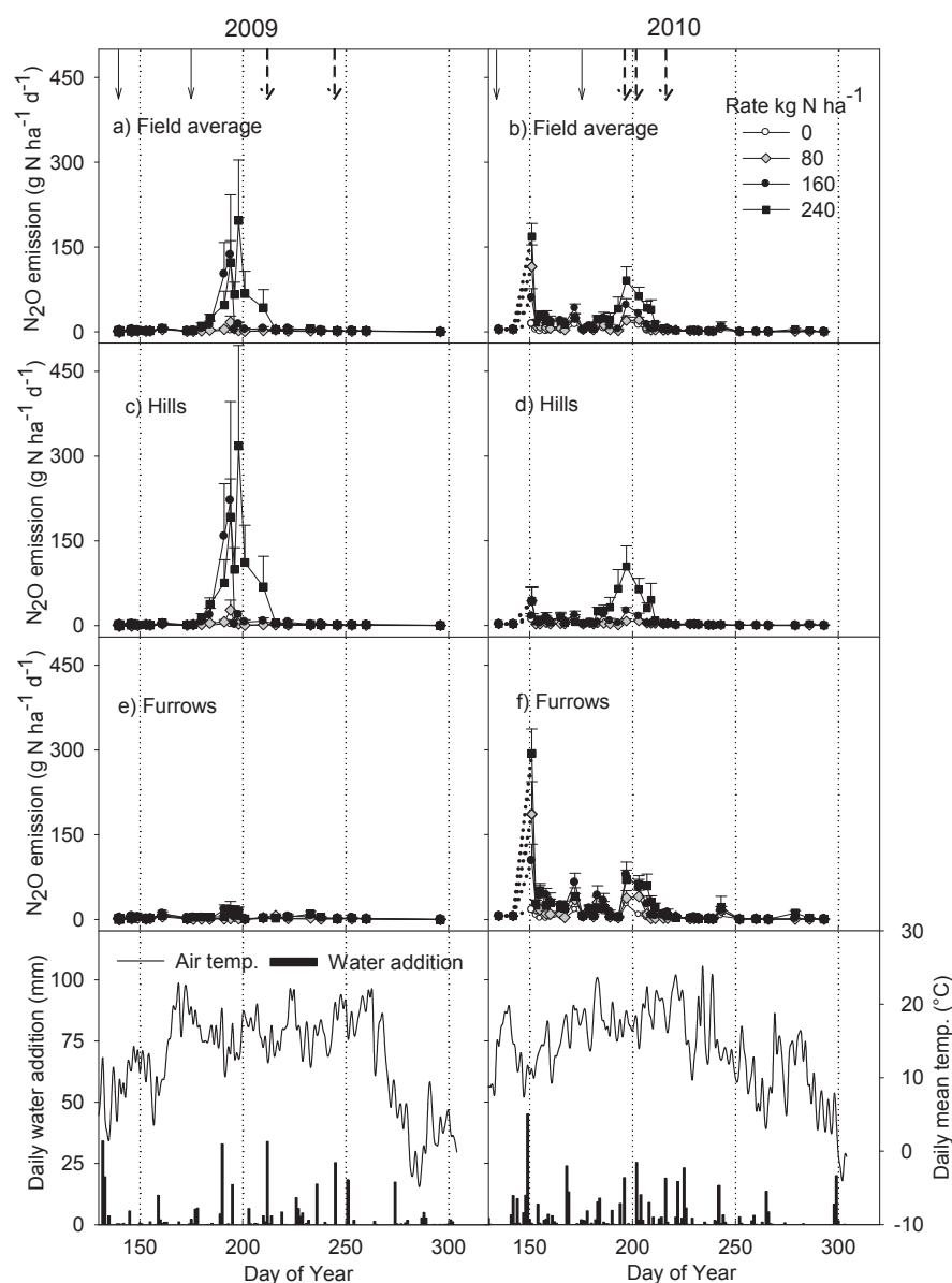
Figure 3. N Rate: Mean daily \text{N}_2\text{O} emissions estimated for treatment plots [average (a, b)], and within plot components, hills (c, d), and furrows (e, f) as affected by fertilizer N rate. Also shown are the average daily air temperature (solid line) and daily water addition (bars, precipitation + irrigation) during the crop seasons in 2009 and 2010. Dotted lines in 2010 indicate the linear interpolation between planting (DOY 135) and the first sampling date (DOY 151). Bars indicate \pm 1 standard error ( n = 8 ) of the mean. The downward solid and dash arrows indicate timing of urea fertilizer additions, and irrigation additions, respectively.
