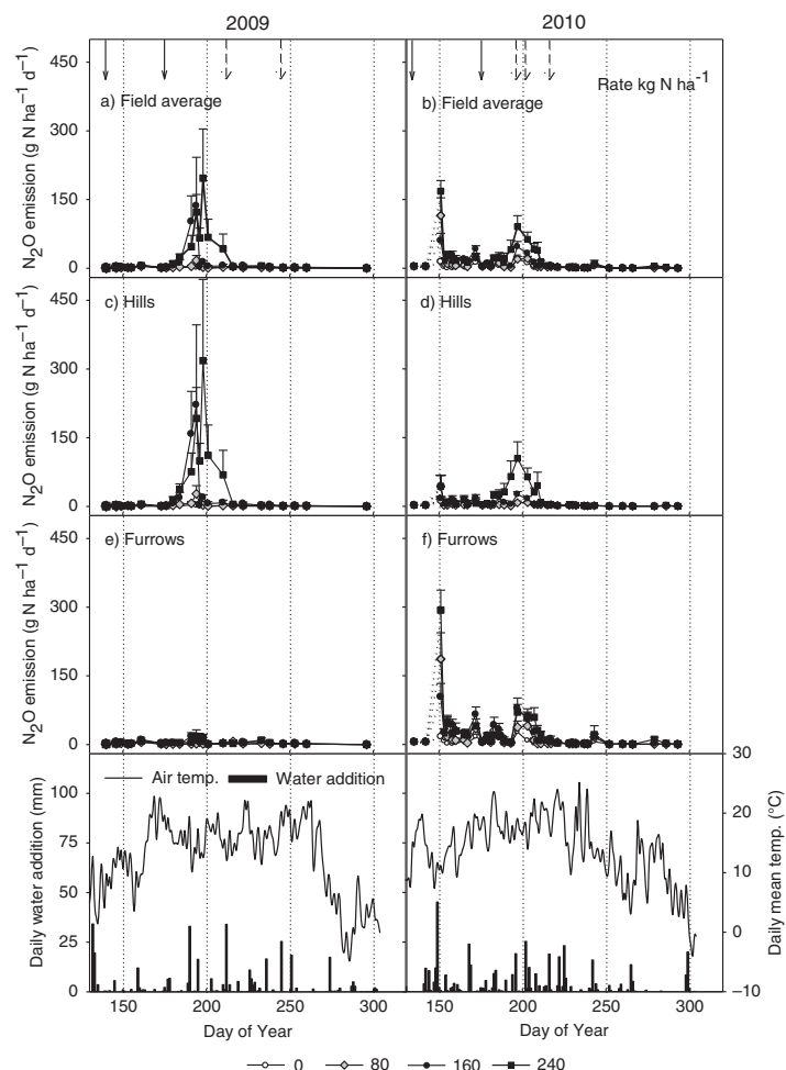
Fig. 1. Mean daily \text{N}_2\text{O} emissions estimated for treatment plots [average (a, b)], and within-plot components, hills (c, d), and furrows (e, f) as affected by fertilizer N rate. Also shown are the average daily air temperature (solid line) and daily water addition (bars, precipitation+irrigation) during the crop seasons in 2009 and 2010. Dotted lines in 2010 indicate the linear interpolation between planting (DOY 135) and the first sampling date (DOY 151). Bars indicate \pm 1 standard error ( n=8 ) of the mean. The downward solid and dash arrows indicate timing of urea fertilizer additions, and irrigation additions, respectively.
